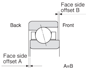
Fig.1.4 Flush grinding
