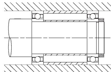
Fig. 5.1 Preloading methods for bearings Fixed position preload
